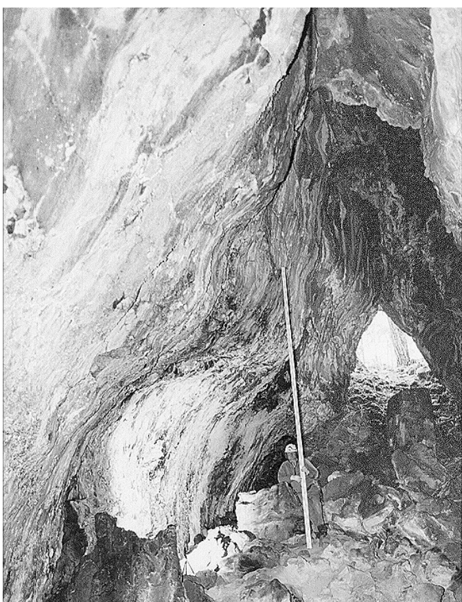
The angular, "gothic", roof of this tube is typical of ones formed by levee overgrowth. (c.f. Figure C →)
