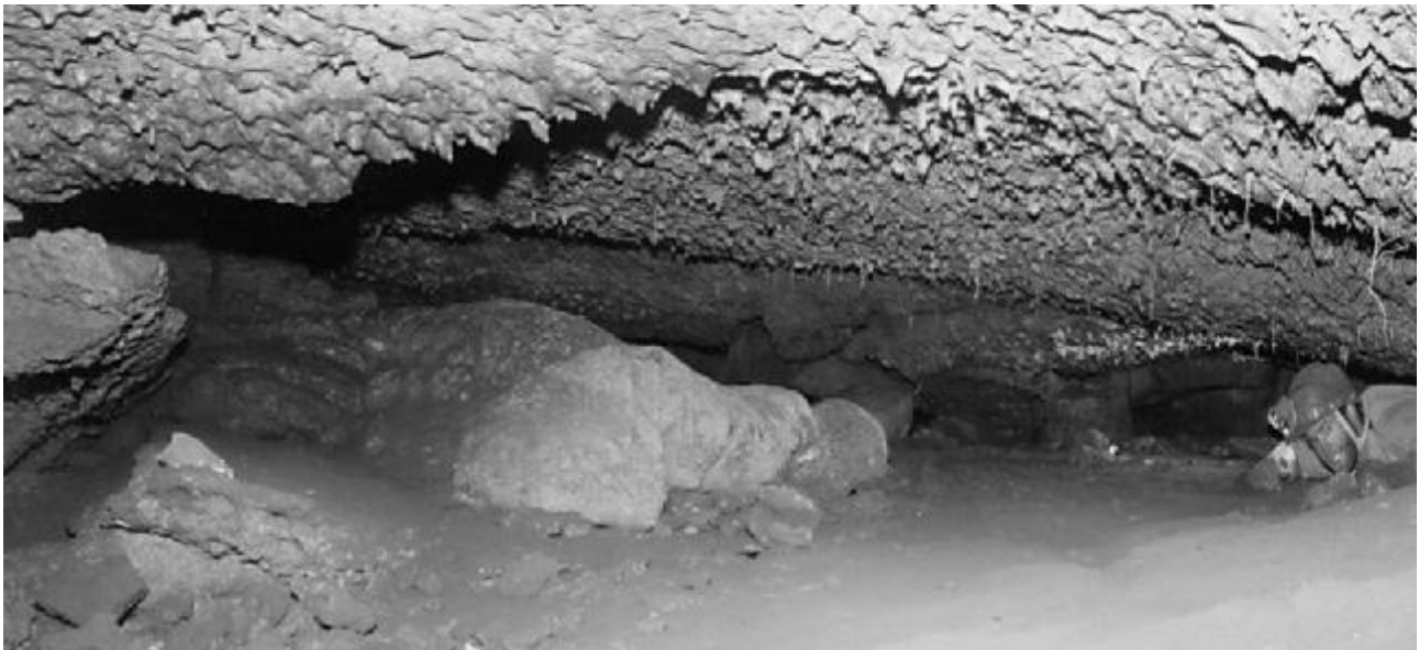
Invasive lava lobe (from left) in second chamber, looking NW. (C0204.10+11)
