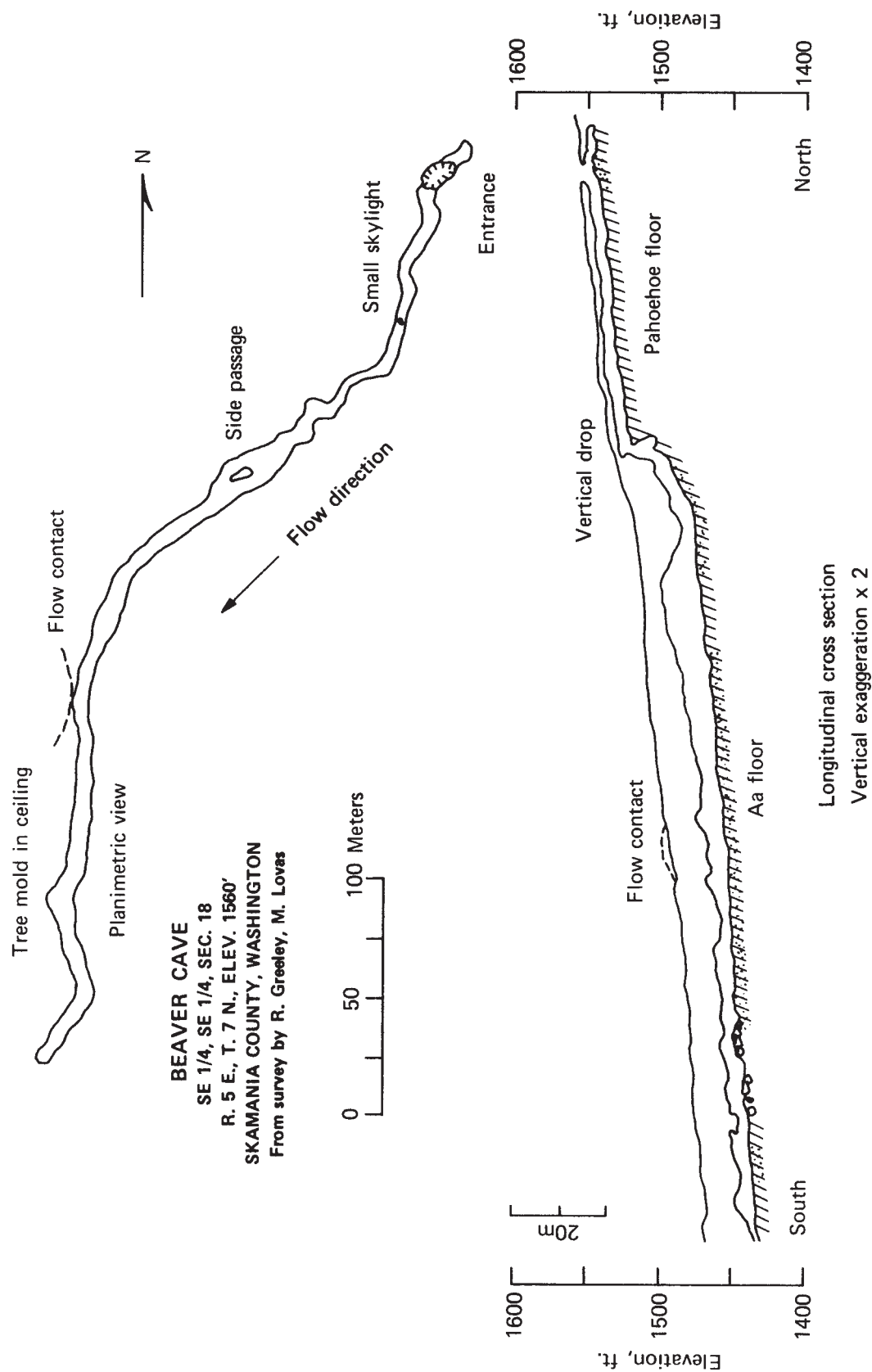
Fig. 11. Cross section and plan view of Beaver Cave.
