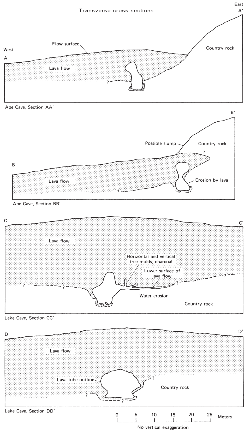
Fig. 14. Transverse cross sections, Mount St. Helens lava tube system, showing relations of lava tube to lava flow and preflow country rock. In these sections, the lava tube is interpreted to occupy a former stream channel.
