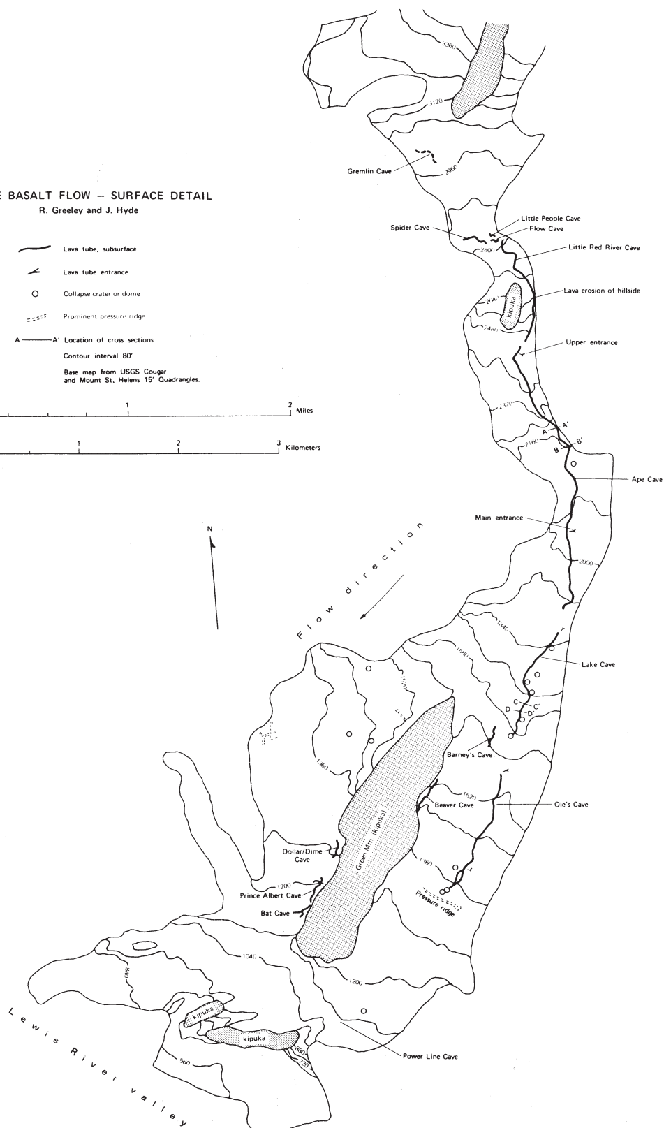
Fig. 6. Topographic map of the Cave Basalt.
