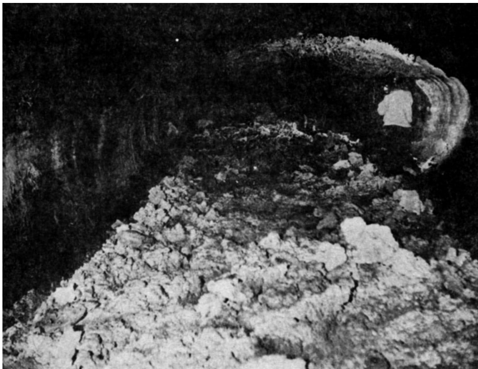
Fig. 21. Spider Cave in which a subsequent floor flow of aa has partially filled the tube interior. Photograph courtesy of C. Larson.
