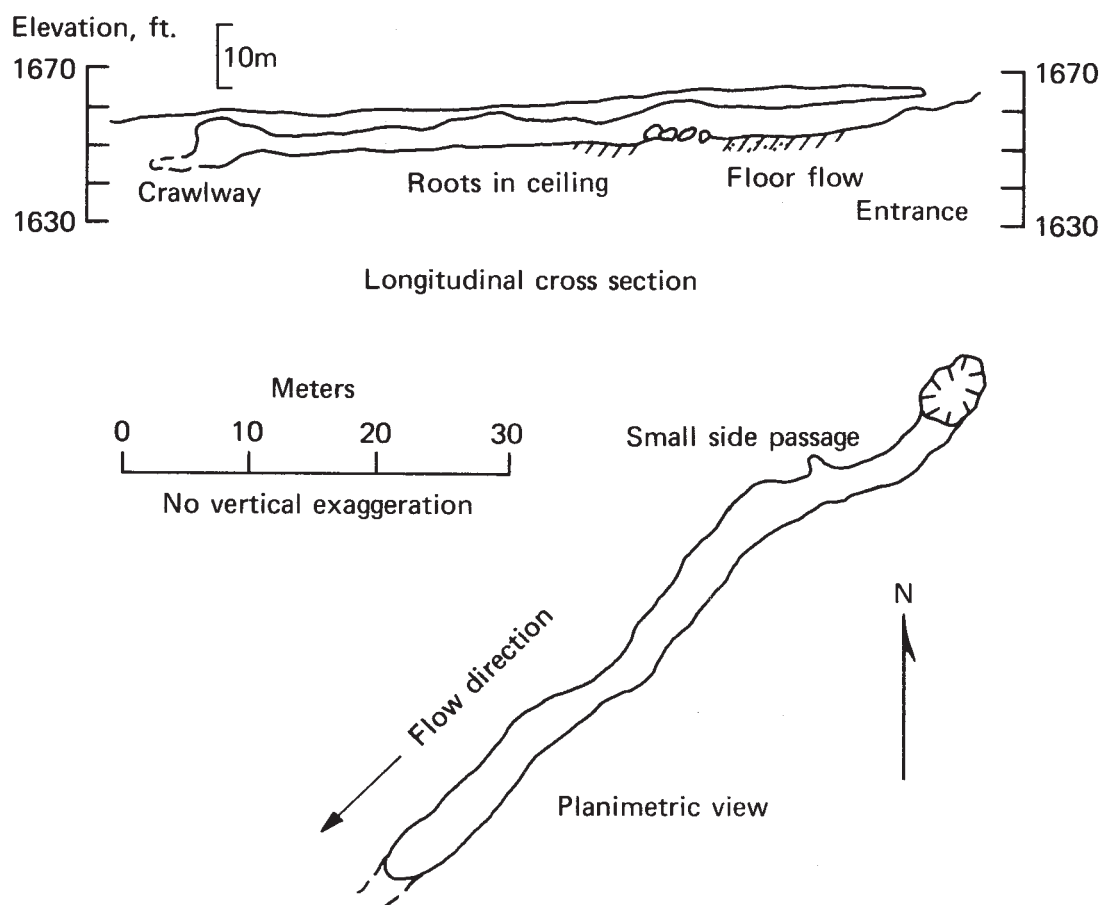
Fig. 12. Cross section and plan view of Barney's Cave.
