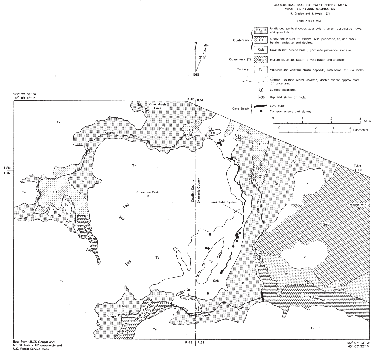
Fig. 2. Geological map of the study area.
