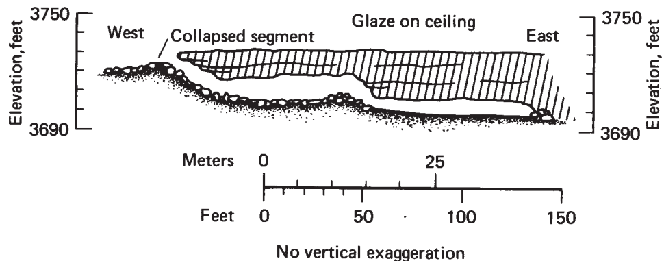
Figure 22. Diagrams of Garbage Caves No. 1 and No. 2, Horse Lava Tube System.
