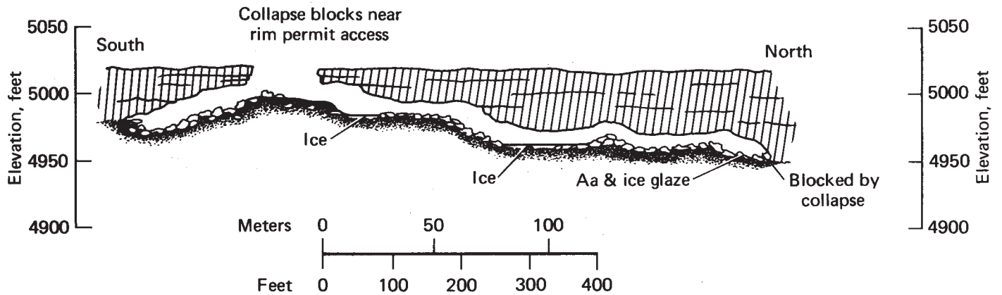
Figure 25. Diagram of South Ice Cave.
